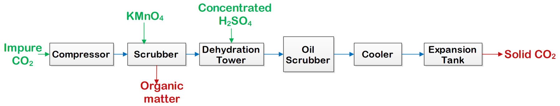
Figure: Manufacturing of High pressure CO 2
